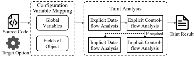
Fig. 5: Framework of CONF-TAINTER.
