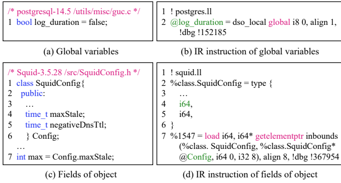
Fig. 4: Examples of configuration variable mapping and the IR instructions.
