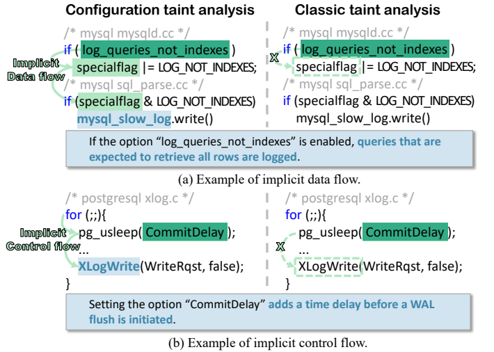
Fig. 1: Example of the difference between configuration taint analysis and classic taint analysis.
